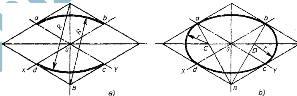
8-shakl. To'g'ri burchakli izometriyada ellips o'rniga oval yasash (2-usul)
